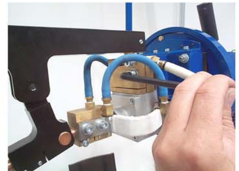
90° electrodes
